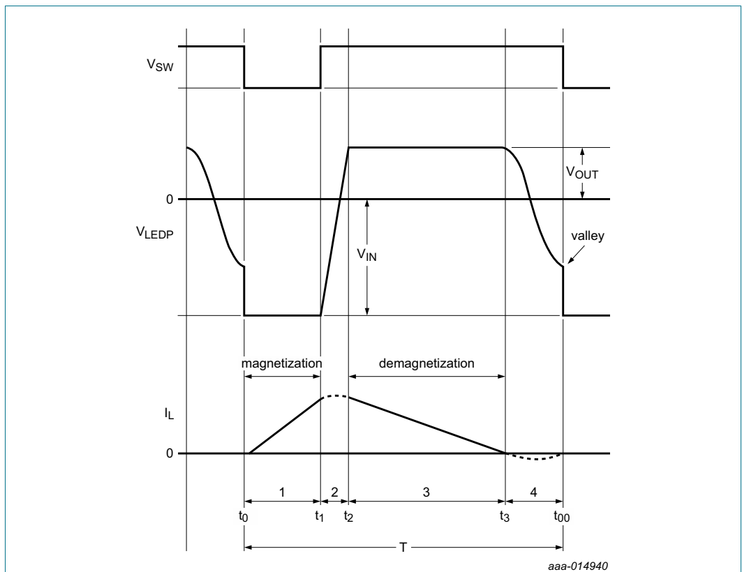
Fig 5. Buck-boost waveforms and valley detection
